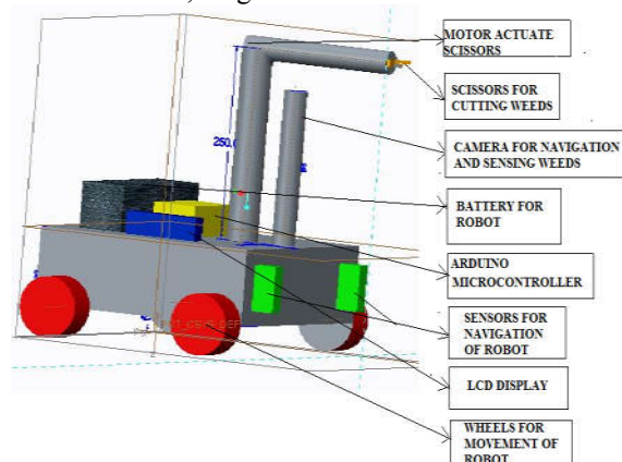
Fig. 1. CAD model of proposed robot
