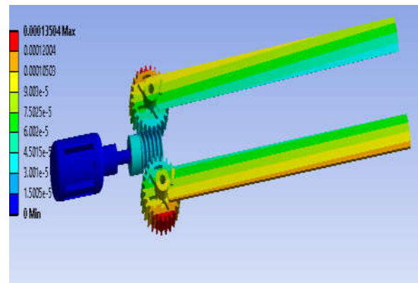
Fig. 7 Total deformation of the cutting mechanism
