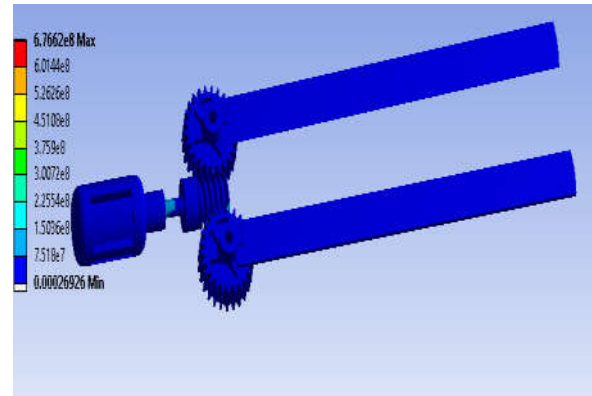
Fig. 6 Equivalent stress on the cutting mechanism
