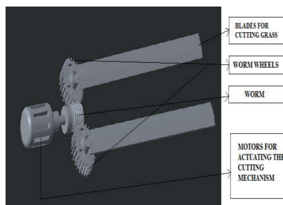
Fig. 2. Cutting mechanism of the deweeding robot
