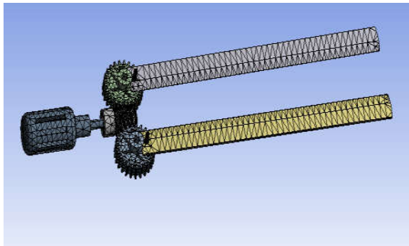
Fig. 3 Meshed part of the cutting mechanism
