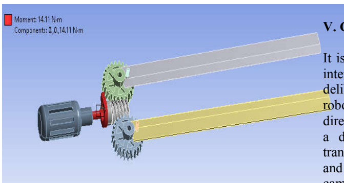
Fig. 5 Moment given to shaft of the motor to rotate worm
