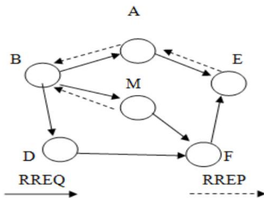
Fig. 1 Routing Discovery Process in AODV Protocol
