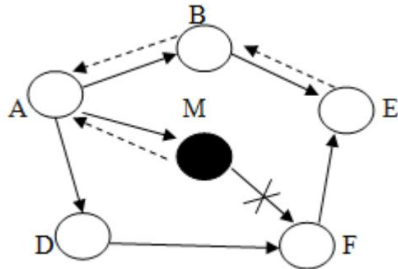
Fig. 2 Black Hole Attack in AODV protocol
