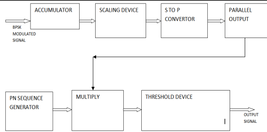
Fig.7: Block diagram of CDMA Receiver
