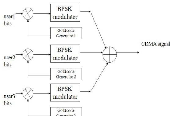
Fig.4. Block diagram of multiple user CDMA transmitters
