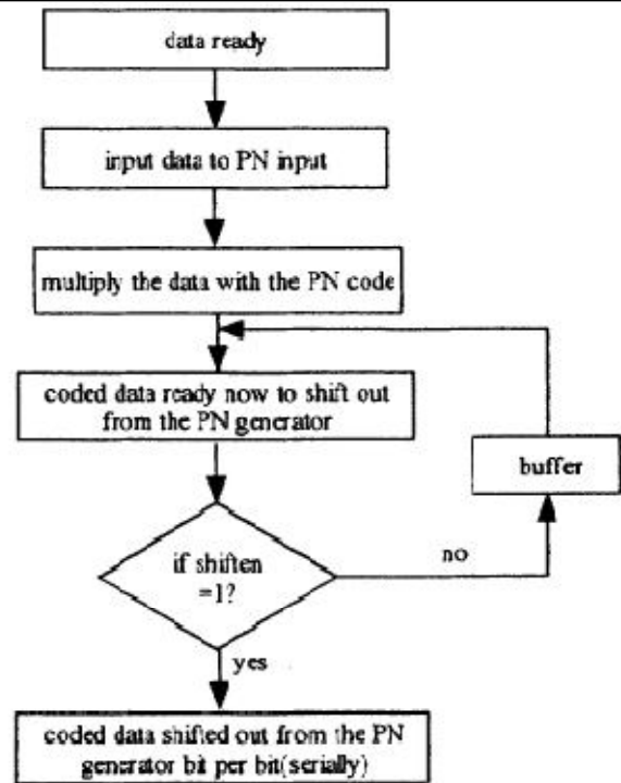
Fig.6. the flow chart of the PN generator
